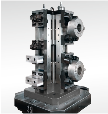
Application example Pallet with clamping device
