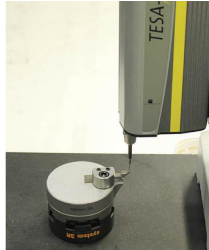
Macro pallet with diamond cutter in a pre-setting station
