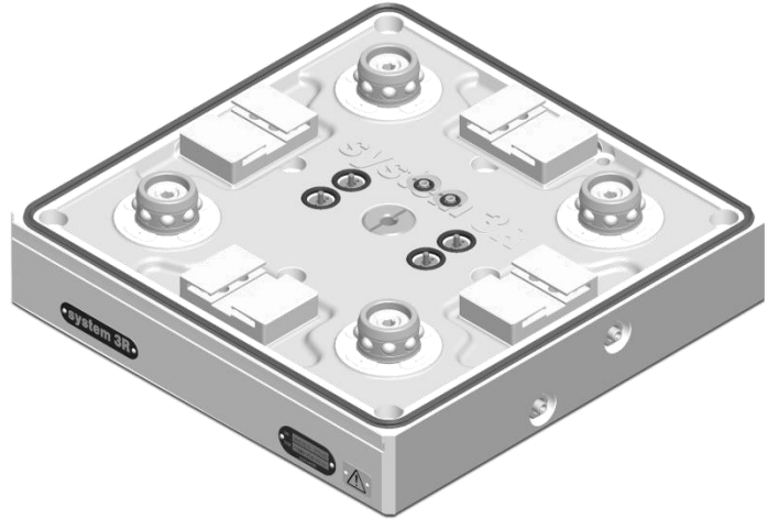
System 3R Dynafix chuck with 4 extra channels.
