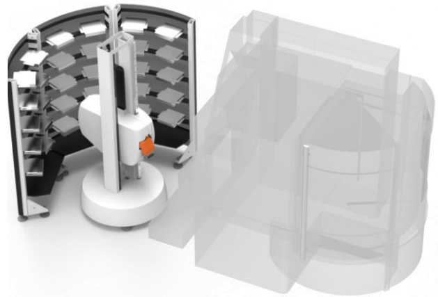
System 3R Transformer robot with one machine
