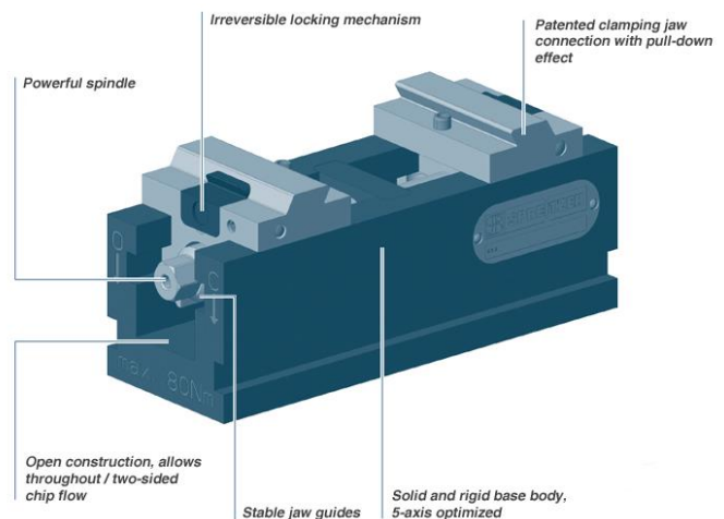
mechanical precise vice, type MZQ
