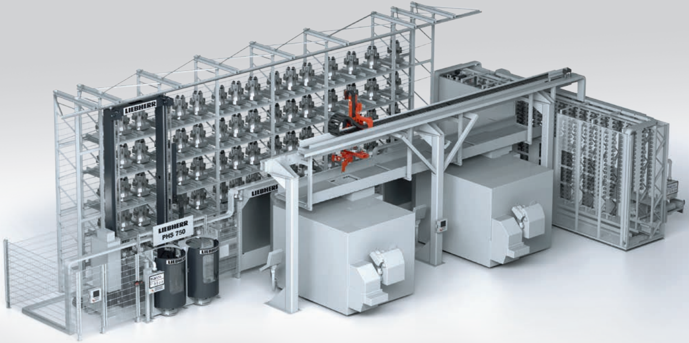
Central Magazine
